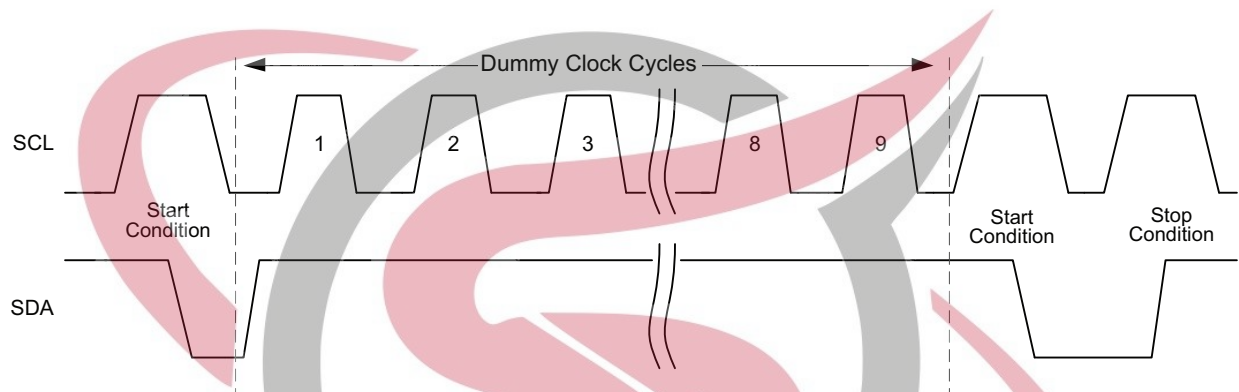
Figure 3-2. Software Reset
